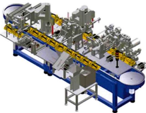
2 Axis Robots
